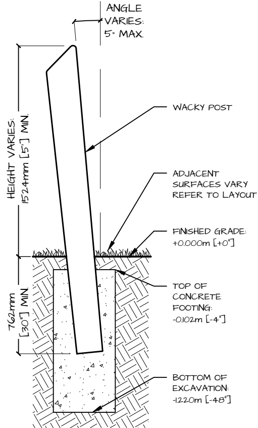
- TYPICAL SECTION -
