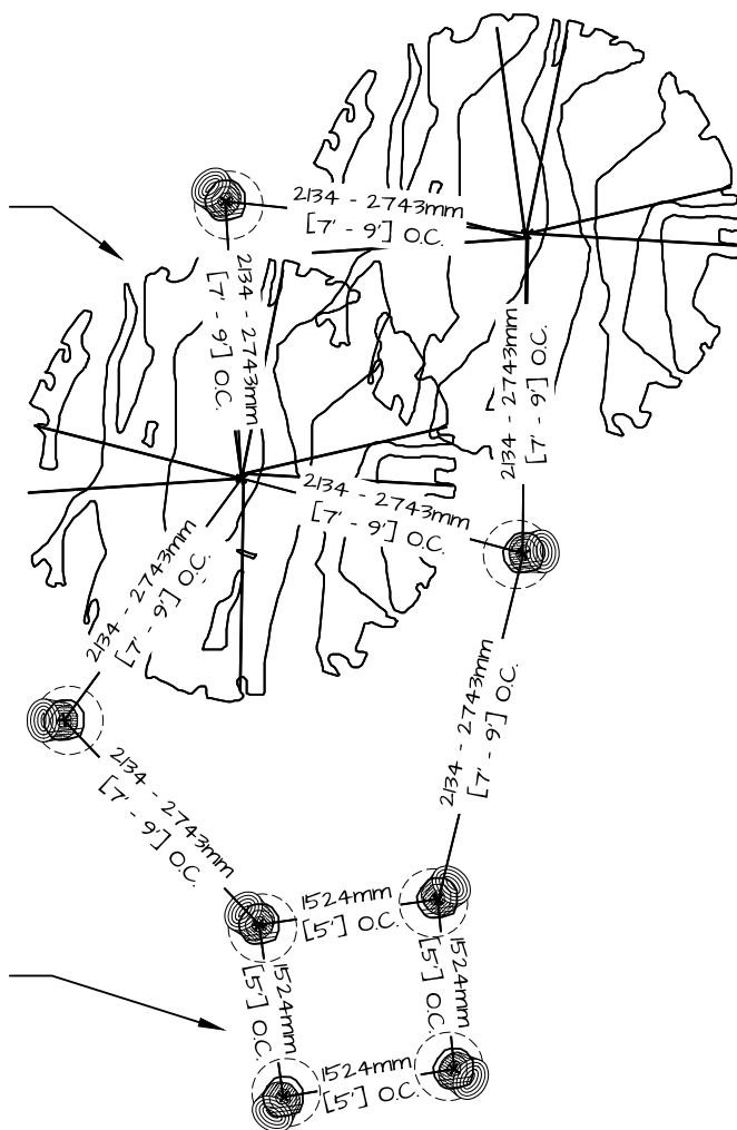
- EXAMPLE LAYOUT PLAN WITH TREES -
